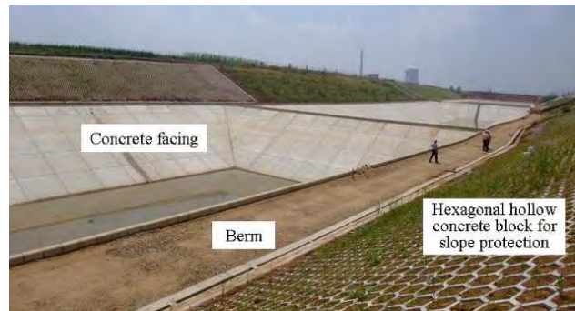
Figure 14 Part of Nanyang test section in expansive soil (Cheng et al. 2011)
